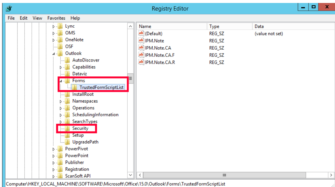
Figure 4: The deployed registry changes
